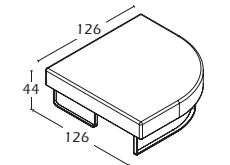
Dimensions: L:126 W:126 H:44 Code: FLU-DWG-CS-F-N-CR Oval Corner, Without Back
