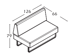
Dimensions: L:126 W:66 H:79 Code: FLU-WAG-RE-F-CR Single Sided Seat, With Back
