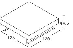
Dimensions: L:126 W:126 H:44,5 Code: FLU-DWG-SQ-F-N-CR Square, Without Back
